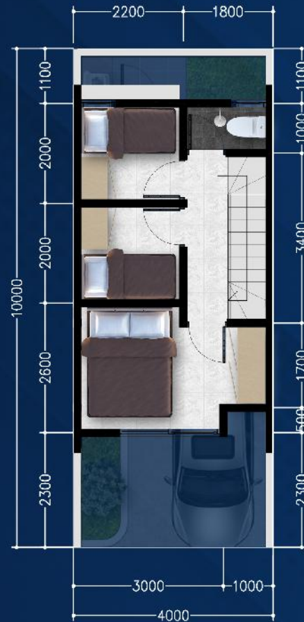
Denah Lantai 2
