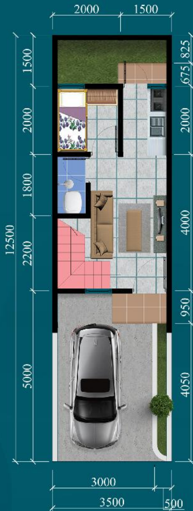
Denah Lantai 1
